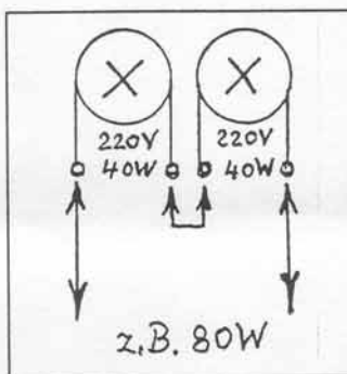
Glühlampen-Dummyload
